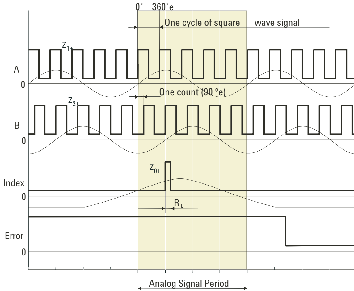
Figure 3. Interpolated digital output signals (A, B, and Index) and the error signal. The analog signal period corresponds to a 40- \mu m distance.
